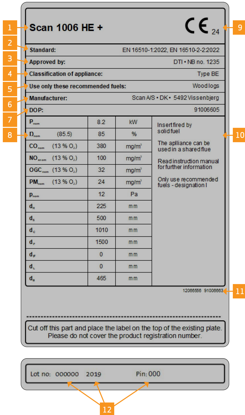
Type plate
